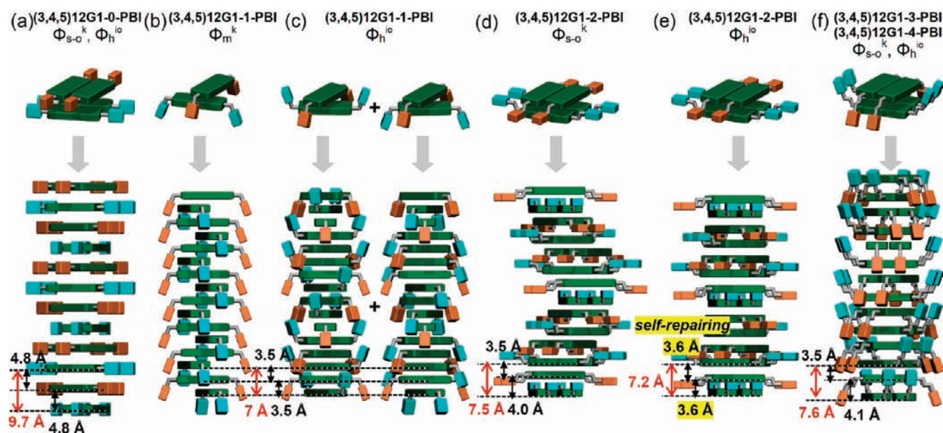
Figure 21. Schematic of the supramolecular columns self-assembled from (3,4,5)12G1- m -PBI ( m = 0, 1, 2, 3, 4 ). In c, the supramolecular columns of the high-temperature \Phi_h^{io} phase are generated by a statistical mixture of the indicated conformations.
