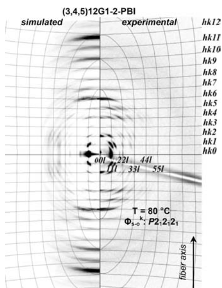
Figure 12. Comparison of the simulated and experimental fiber patterns of (3,4,5)12G1-2-PBI collected at 80^\circ\text{C} in the \Phi_{s-o}^k phase.
