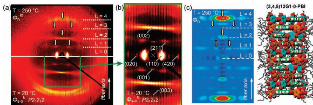
Figure 5. Wide-angle XRD patterns collected from the oriented fiber of (3,4,5)12G1-0-PBI (a, b), simulation of the WAXS fiber pattern and molecular model of the supramolecular column (c). For clarity, the pattern from b is shown with higher contrast. In a and c, the vertical arrows indicate the layer line principal maxima identified in the high-temperature \Phi_{h^{io}} phase. Color code used in the molecular model from c: O atoms, red; H atoms, white; N atoms, blue; C atoms of the PBI, green; C atoms of the dendron phenyl, orange and light blue (Figure 6); all other C atoms, gray.
