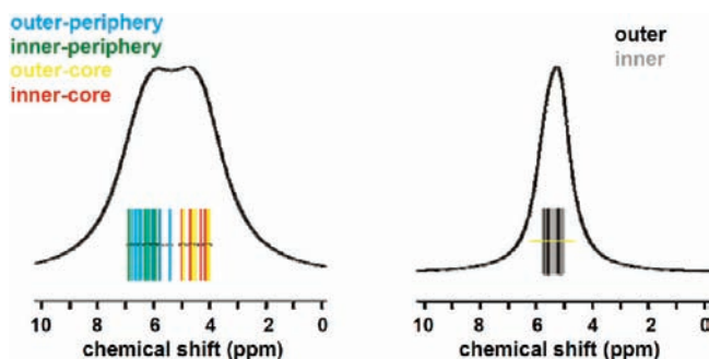
Figure 24. Calculated chemical shift distribution for (3,4,5)12G1-2-PBI along an ab initio molecular dynamics trajectory (left). The individual NMR chemical shifts were convoluted with Gaussians to yield a continuous spectrum. Prior to the convolution, all inner and all outer hydrogen atoms were averaged, which corresponds to the effects of a flip-exchange process (right).
