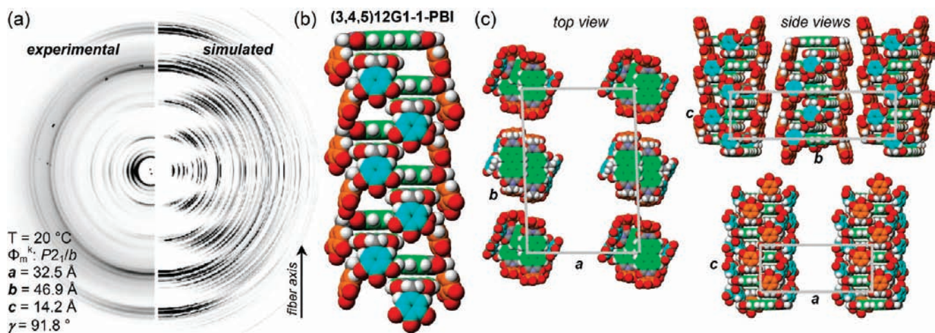
Figure 8. Comparison of the experimental and simulated XRD patterns collected from the oriented fiber of (3,4,5)12G1-1-PBI at 20 °C in the columnar monoclinic crystalline phase, \Phi_m^k (a), and detail of the molecular model used in the simulation (b, c).
